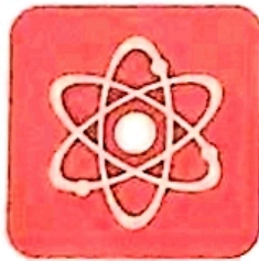
PHYSICS
