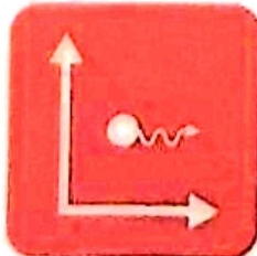
QUANTUM MECHANICS
